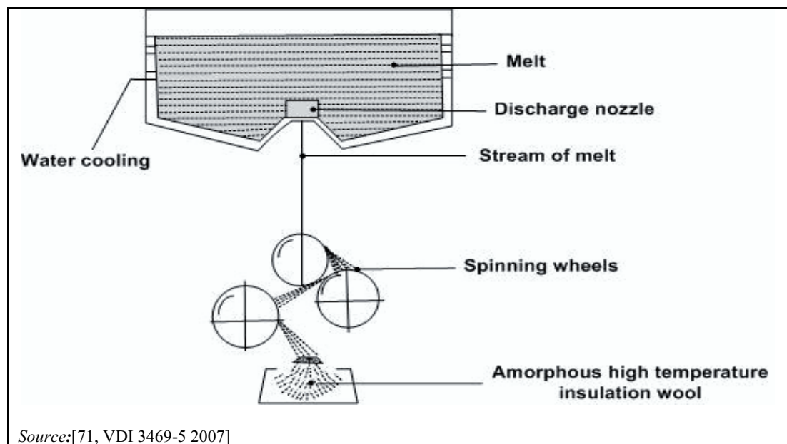
Figure 2.16: Spinning process
