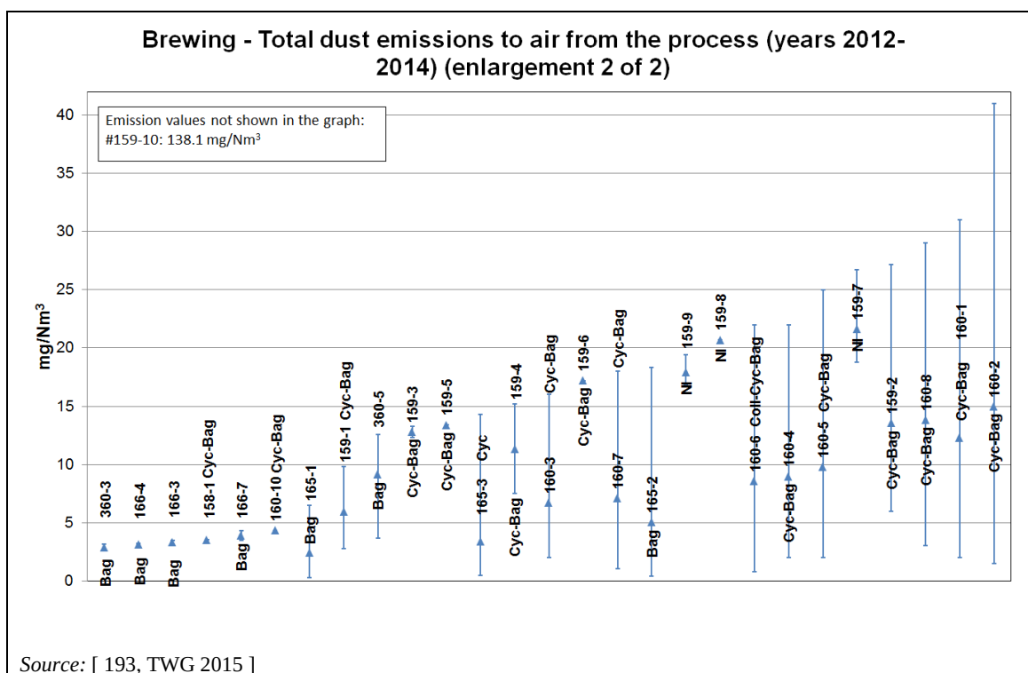
Figure 4.17: Total dust emissions to air from the brewing process (2 of 2)
