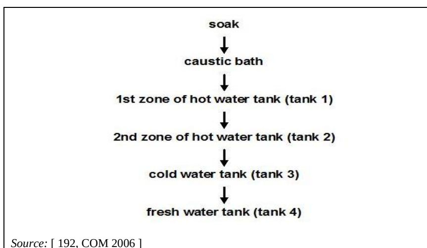
Figure 4.11: Bottle cleaning and rinsing steps
