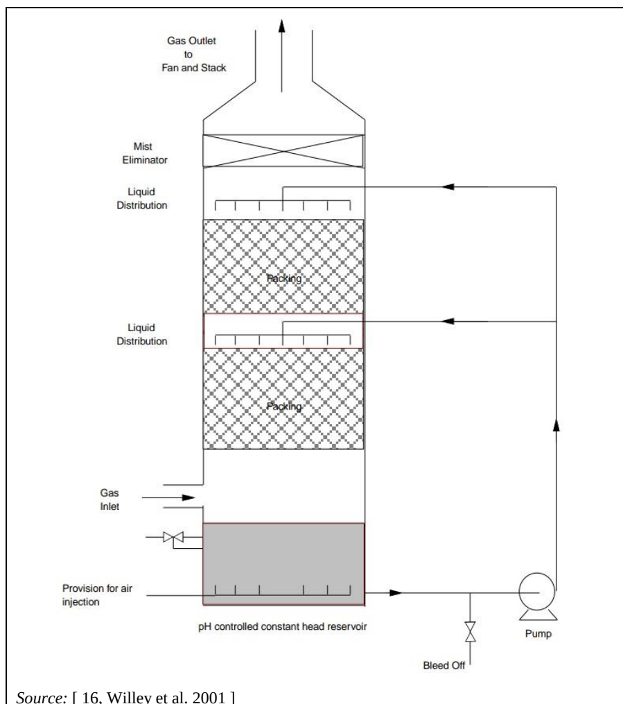
Figure 2.49: Bioscrubber layout
