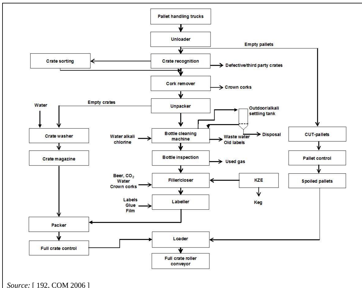
Figure 2.13: A CIP system for the bottling process in a brewery
