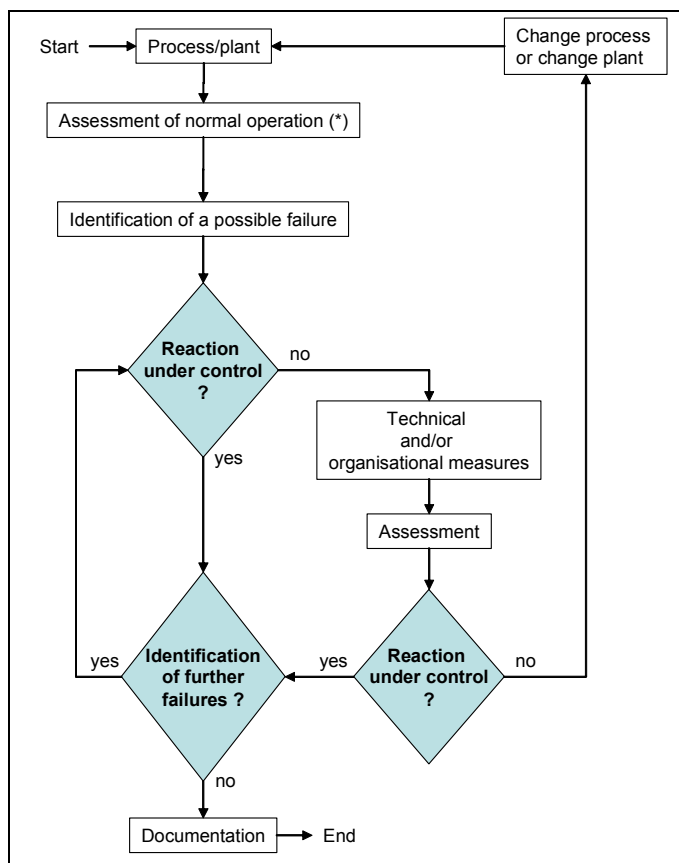
Figure 4.7: Safety assessment procedure Note: (*) see Figure 4.8
