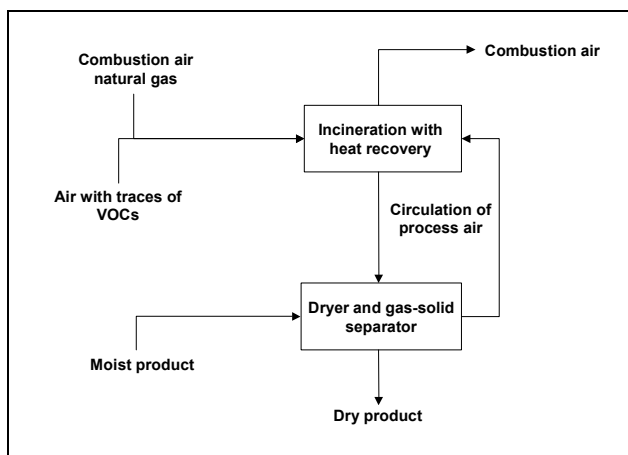
Figure 4.4: Incineration of process air containing Volatile Organic Compounds (VOCs)
