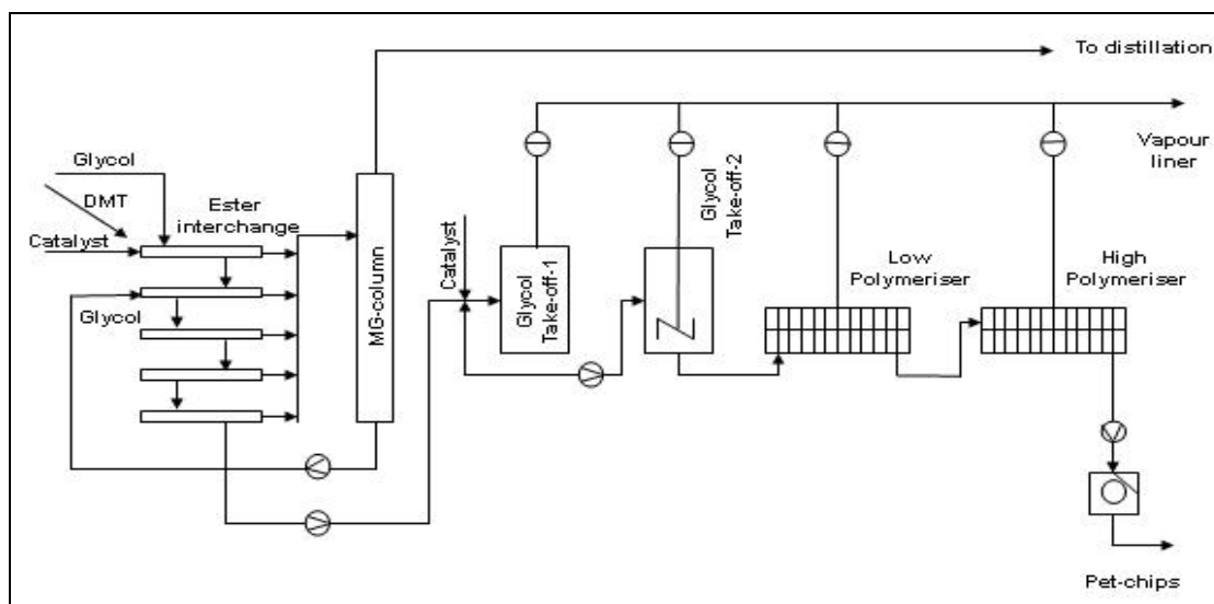
Figure 10.2: Flow chart of the PET DMT process
