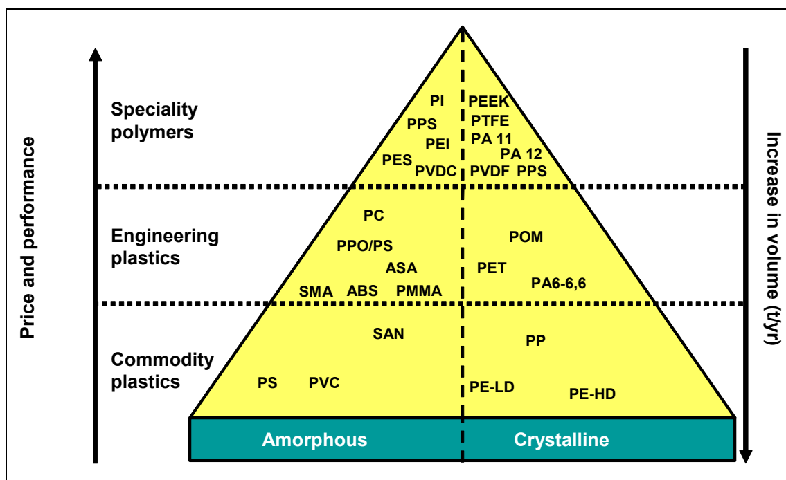
Figure 1.6: Classification of thermoplastic polymers
